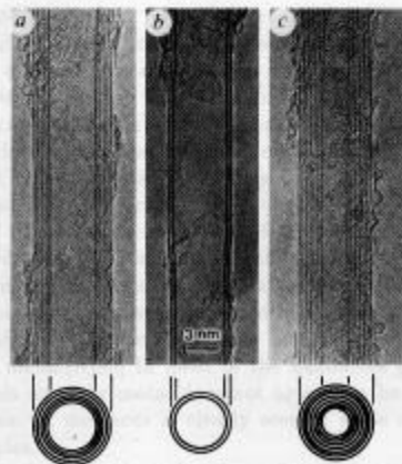
FIG. 1 Electron micrographs of microtubules of graphitic carbon. Parallel dark lines correspond to the (002) lattice images of graphite. A cross-section of each tube is illustrated. a, Tube consisting of five graphitic sheets, diameter 6.7 nm. b, Two-sheet tube, diameter 5.5 nm. c, Seven-sheet tube, diameter 6.5 nm, which has the smallest hollow diameter (2.2 nm).
