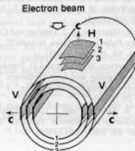
FIG. 2 Cinographic view of a possible structural model for a graphitic tube. Each cylinder represents a coaxial closed layer of carbon hexagons. The meaning of the labels V and H is explained in the text.
