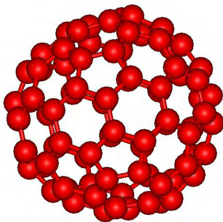
C_{84} - D_{2d}
