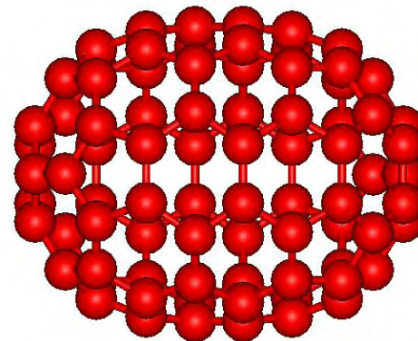
C_{80} - D_{5d}
